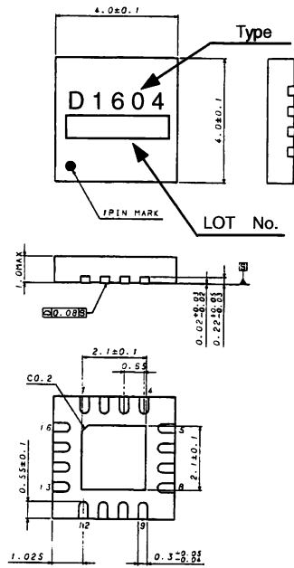
SQFN016V4040 (16PIN) (Unit : mm)
