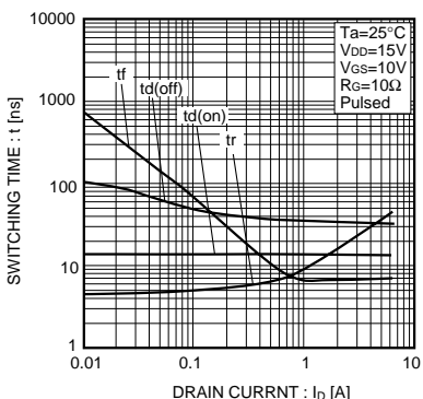
Fig.9 Switching Characteristics
